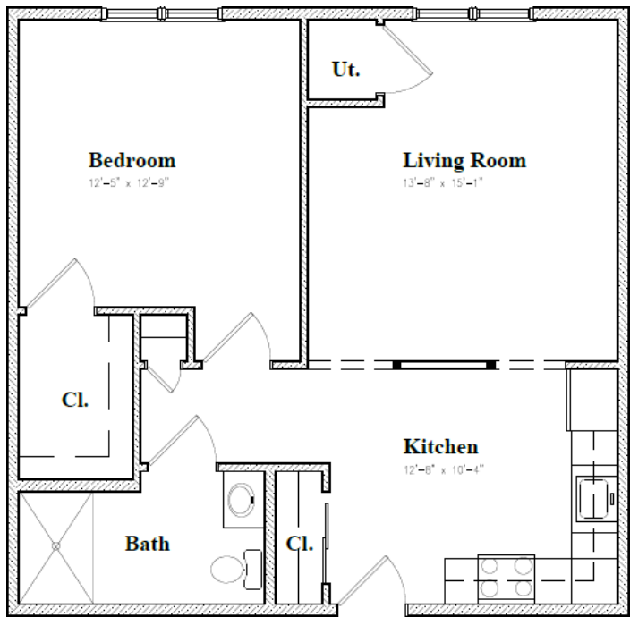
1 Bedroom Layout 706 sq. ft.
